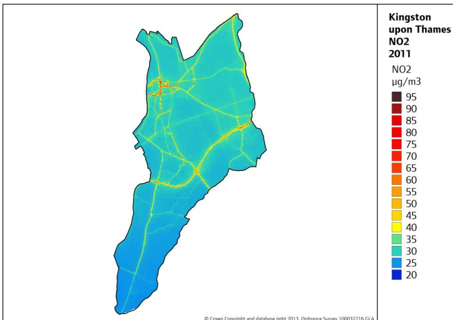
Image 6 Annual mean concentrations of NO 2 in LB Kingston upon Thames 2011
