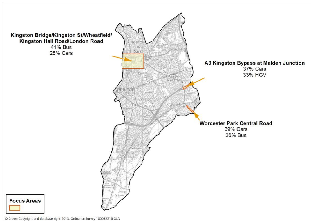
Image 4 – LB Kingston upon Thames Focus Areas and Air Quality Monitors, London Atmospheric Emissions Inventory
