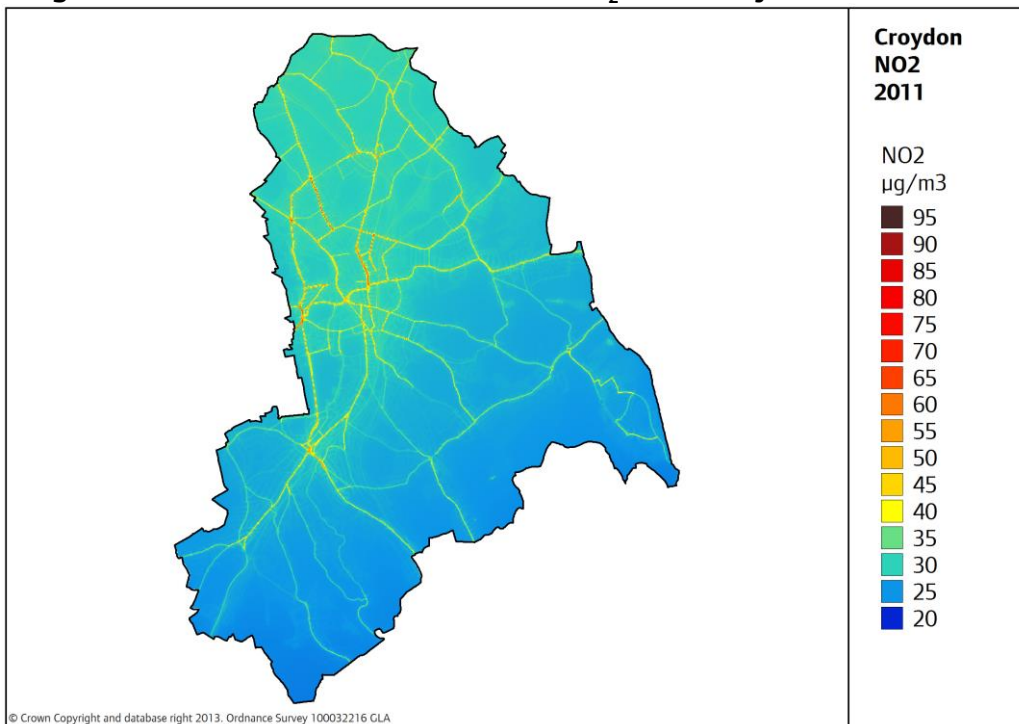
Image 6 Annual mean concentrations of NO 2 in LB Croydon 2011
