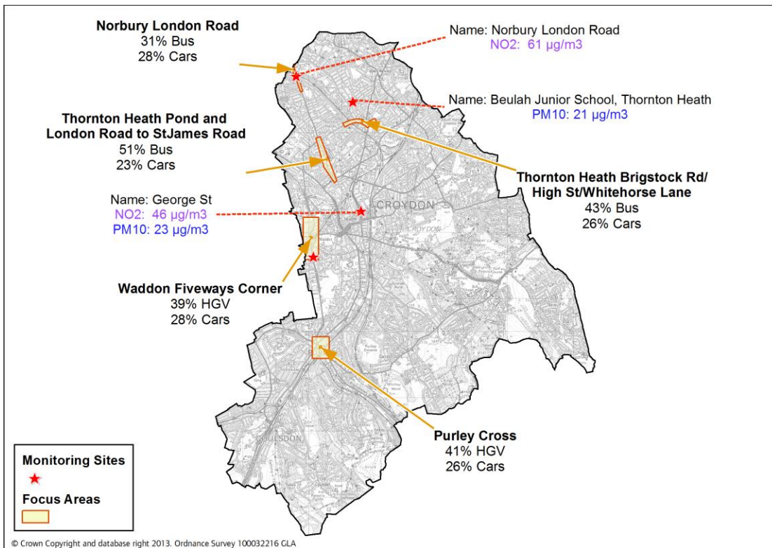
Image 4 – LB Croydon Focus Areas and Air Quality Monitors, London Atmospheric Emissions Inventory
