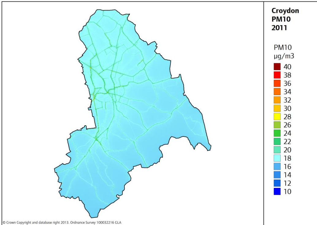
Image 5 Annual mean concentrations of PM 10 in LB Croydon 2011
