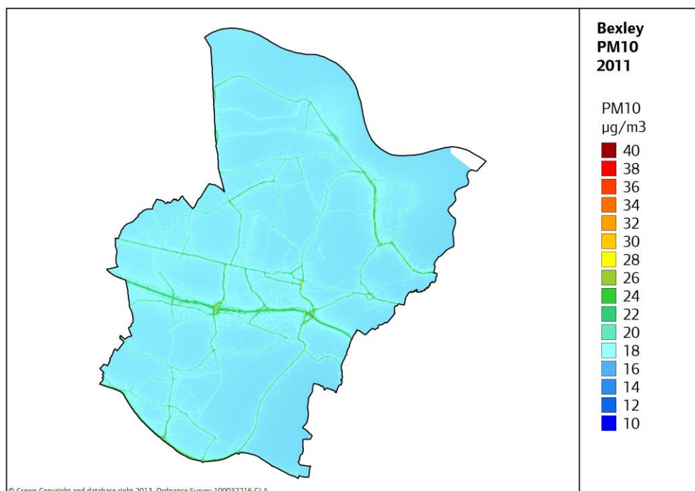
Image 5 Annual mean concentrations of PM 10 in LB Bexley 2011
