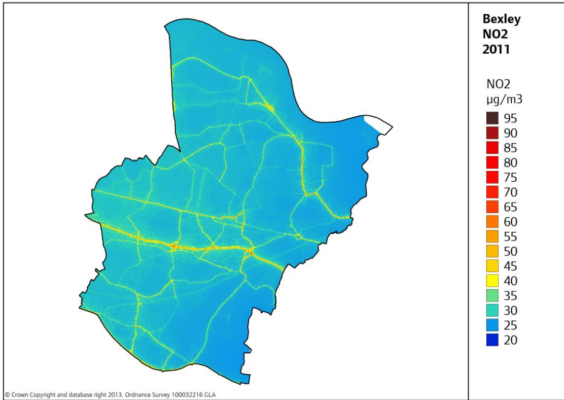
Figure 6 Annual mean concentrations of NO 2 in LB Bexley 2011
