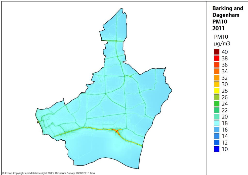
Image 5 Annual mean concentrations of PM 10 in LB Barking & Dagenham 2011
