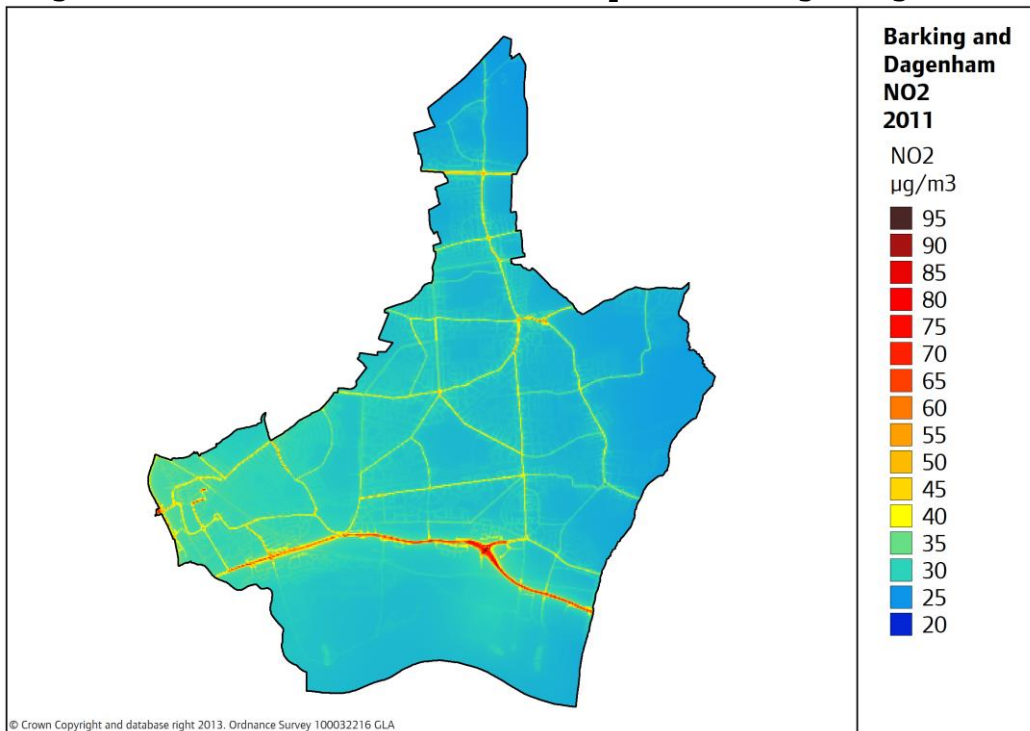
Image 6 Annual mean concentrations of NO 2 in LB Barking & Dagenham 2011
